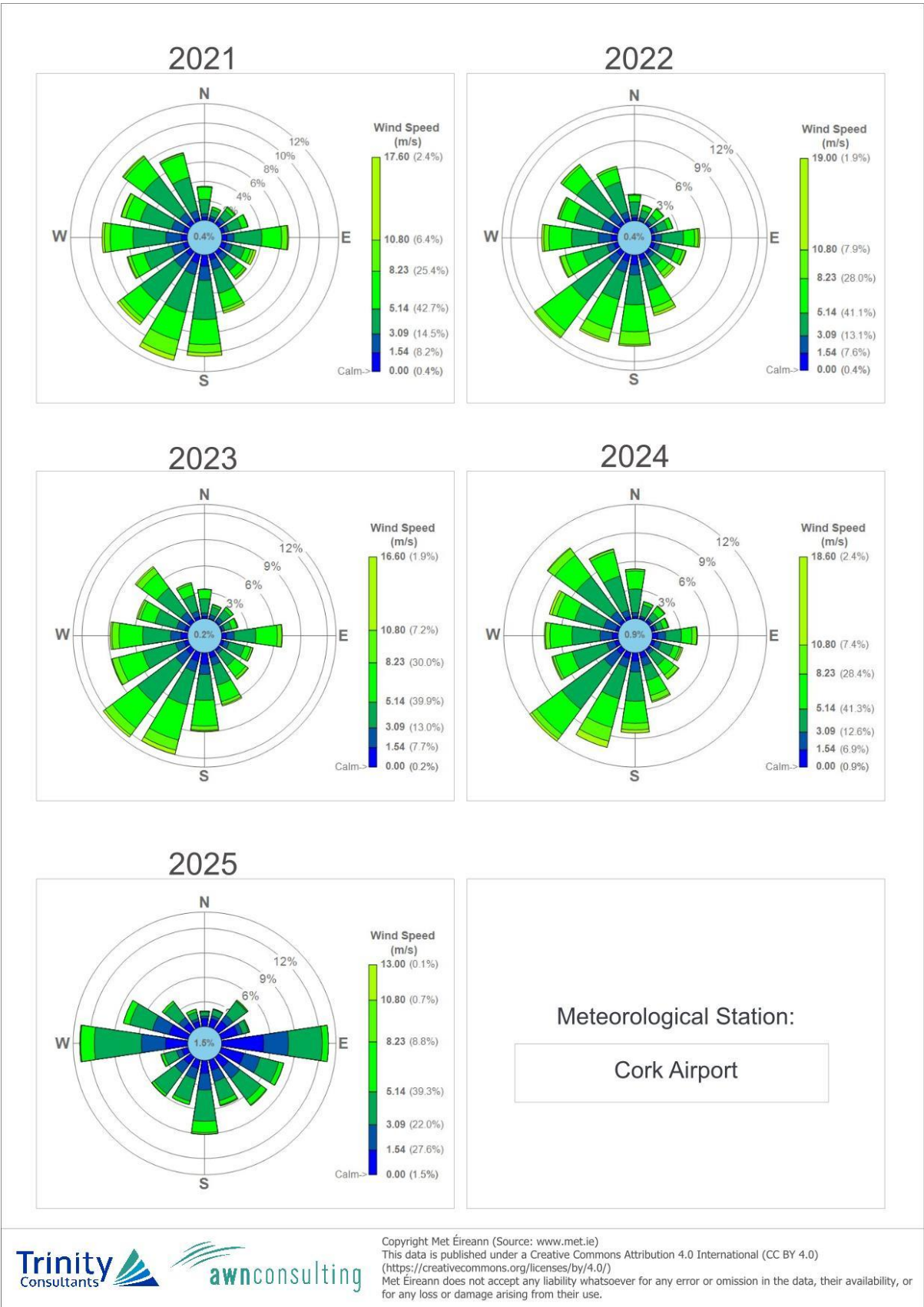
Figure 8.4 Cork Airport Windrose 2021 -2025
