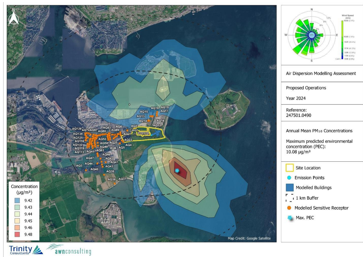
Figure 8.17 Maximum Operations: Predicted PM 10 Annual Concentrations
