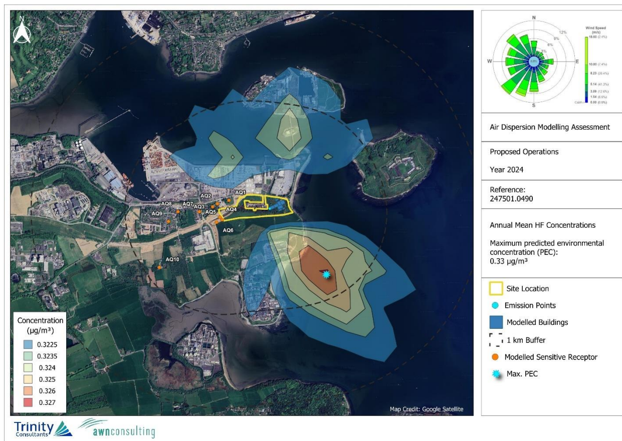
Figure 8.22 Maximum Operations: Predicted HF Annual Average Concentration
